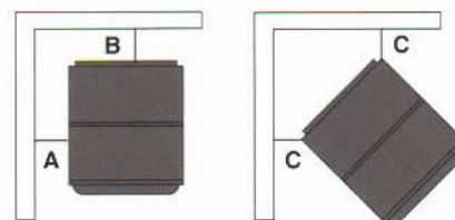
Minimum Clearances to Combustible Materials
