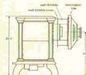
Components for a minimum horizontal vent configuration
