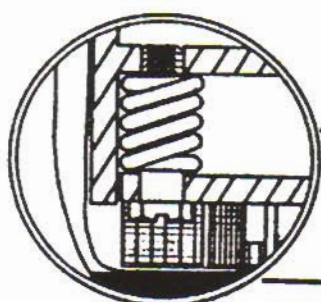
Snap Spring Assembly for cleaning secondary filter without taking off lid.
